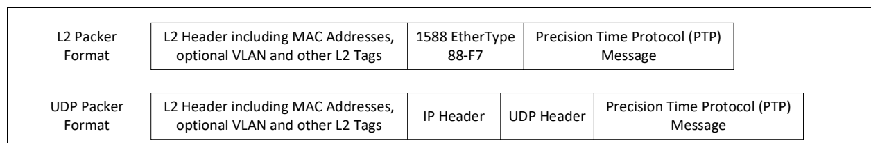
Figure 8-14. 1588 Packet Format
